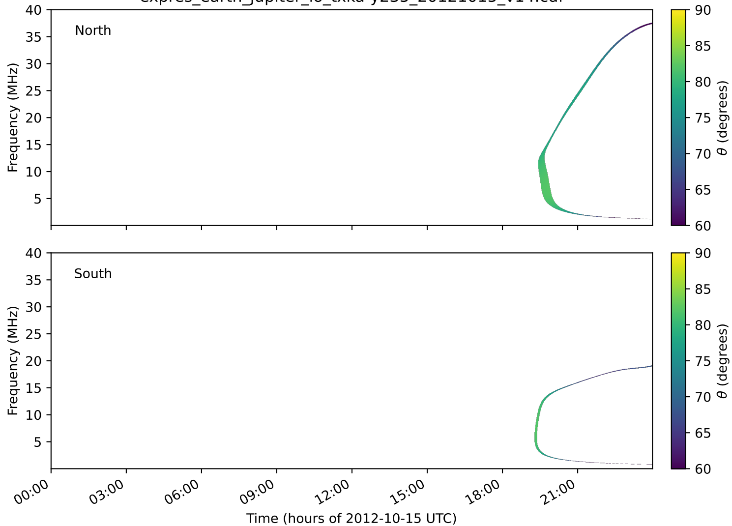
expres_earth_jupiter_io_txka-y235_20121015_v14.cdf
