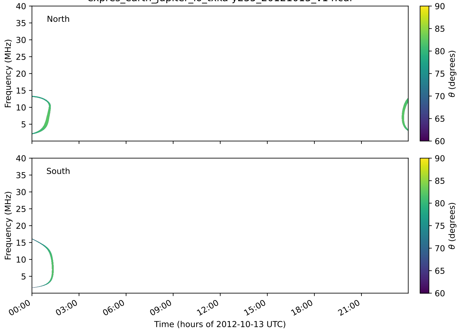
expres_earth_jupiter_io_txka-y235_20121013_v14.cdf
