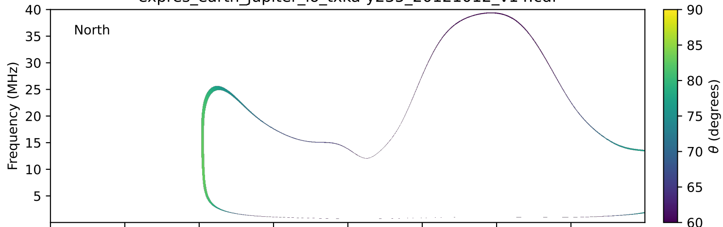
expres_earth_jupiter_io_txka-y235_20121012_v14.cdf
