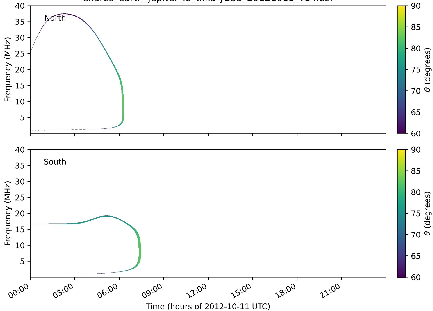
expres_earth_jupiter_io_txka-y235_20121011_v14.cdf
