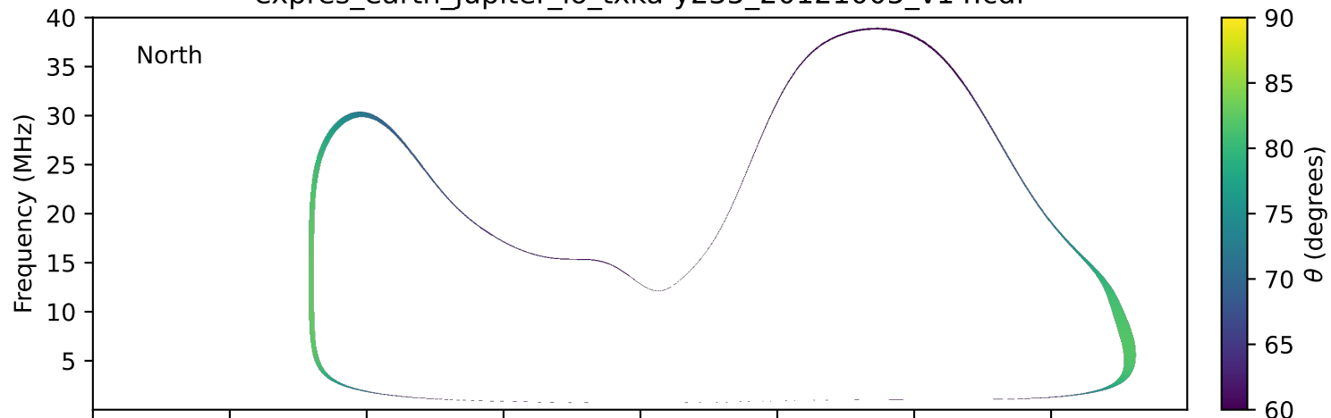
expres_earth_jupiter_io_txka-y235_20121005_v14.cdf
