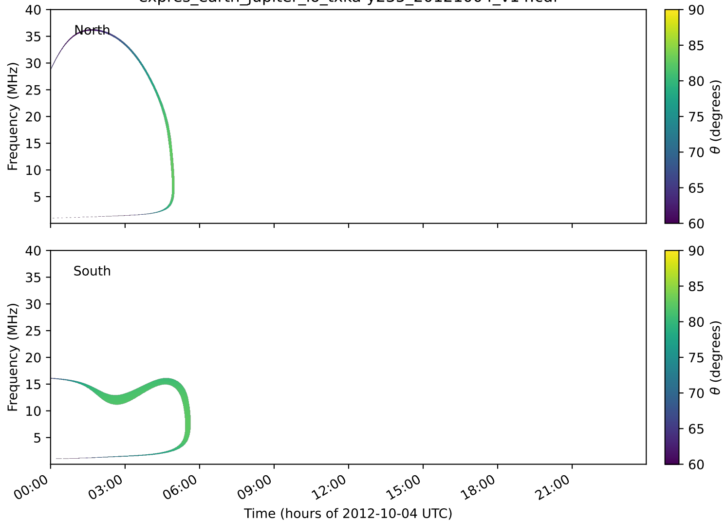
expres_earth_jupiter_io_txka-y235_20121004_v14.cdf
