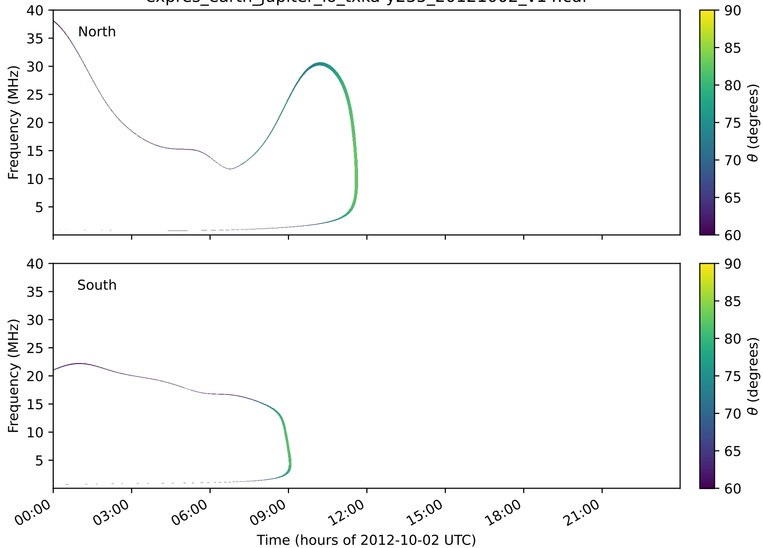
expres_earth_jupiter_io_txka-y235_20121002_v14.cdf
