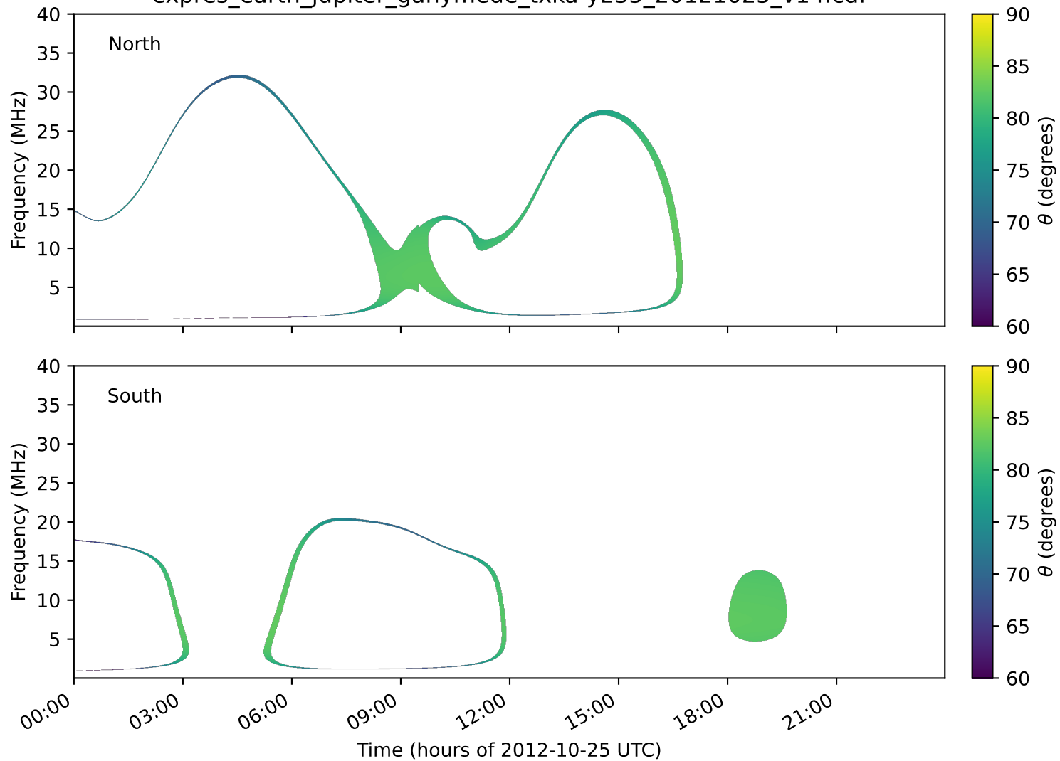
expres_earth_jupiter_ganymede_txka-y235_20121025_v14.cdf
