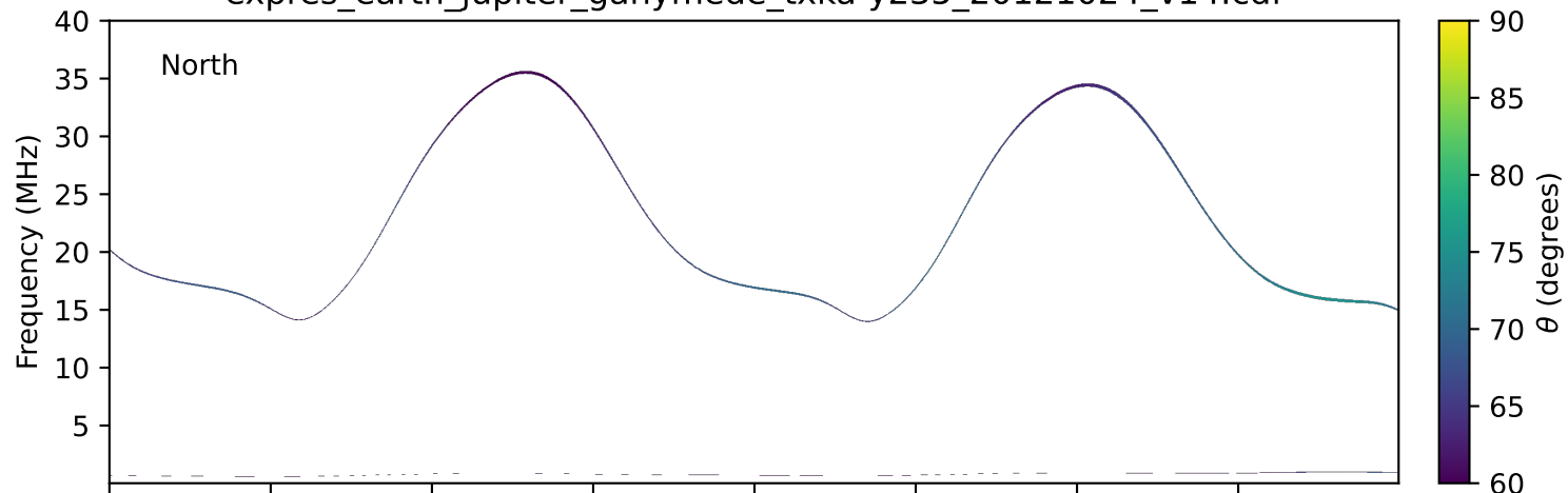
expres_earth_jupiter_ganymede_txka-y235_20121024_v14.cdf
