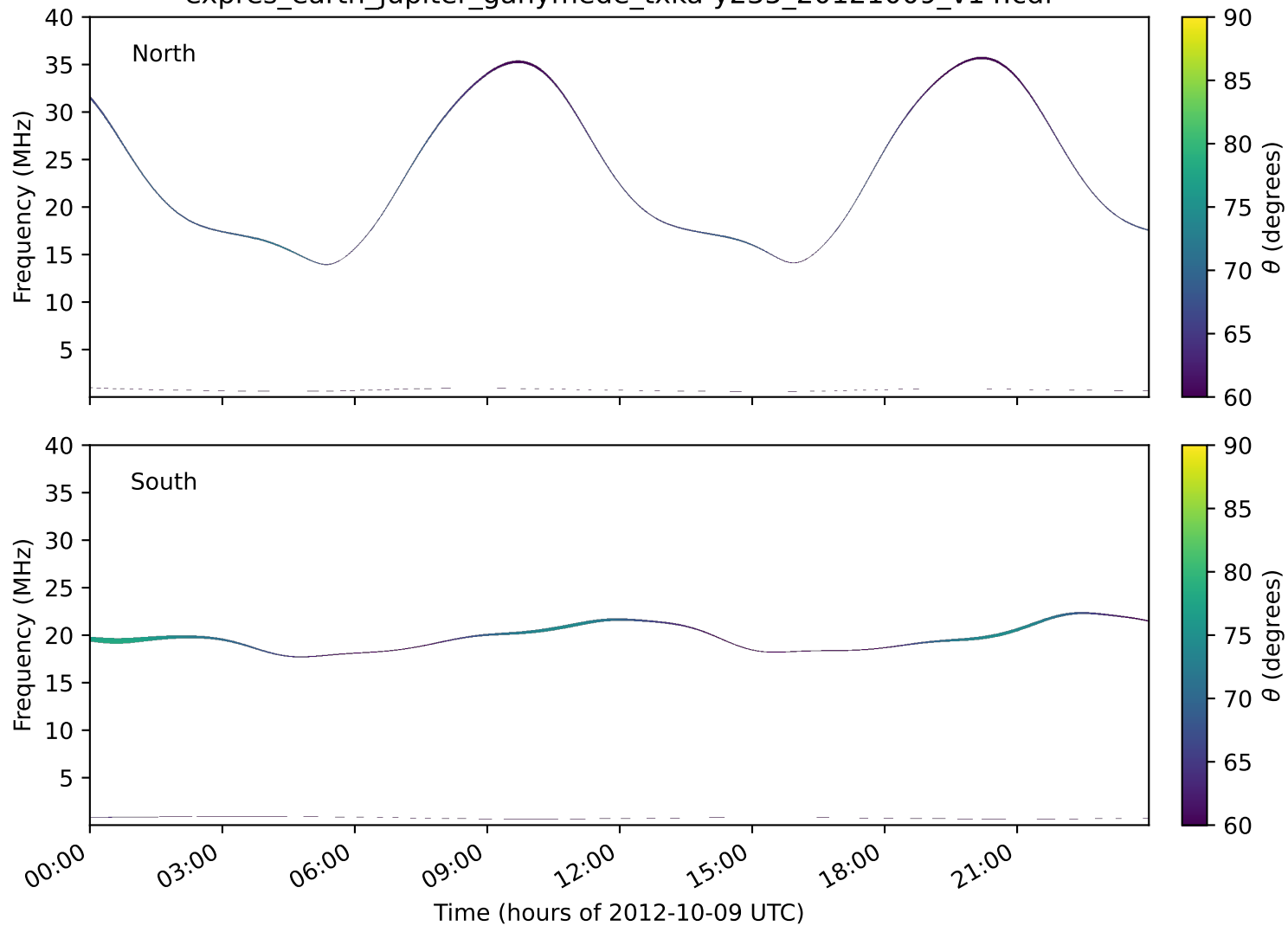
expres_earth_jupiter_ganymede_txka-y235_20121009_v14.cdf
