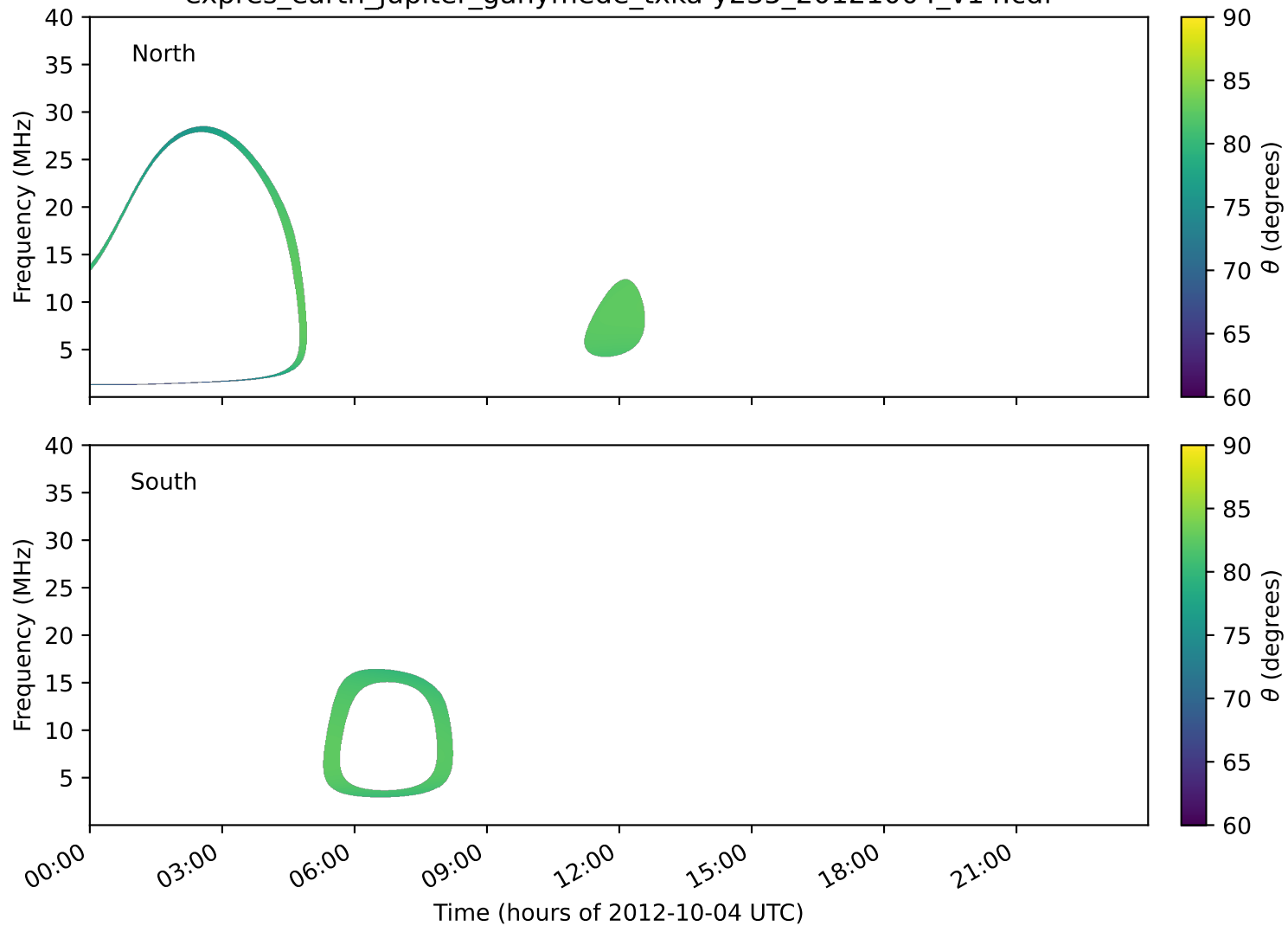
expres_earth_jupiter_ganymede_txka-y235_20121004_v14.cdf
