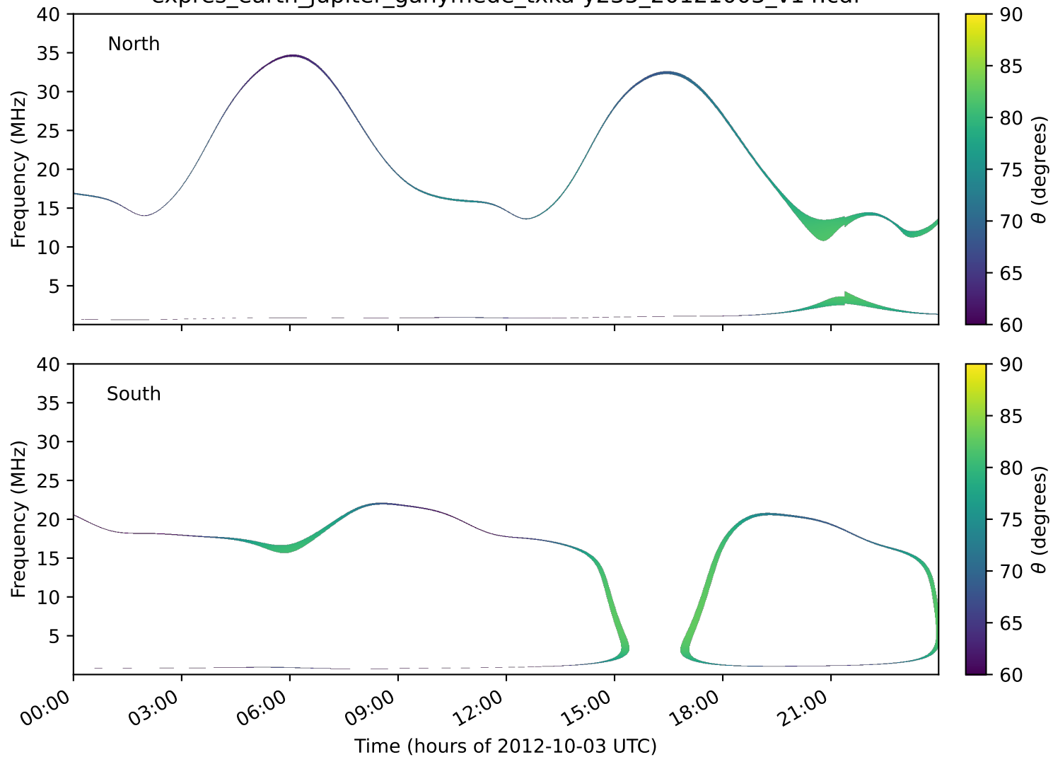
expres_earth_jupiter_ganymede_txka-y235_20121003_v14.cdf
