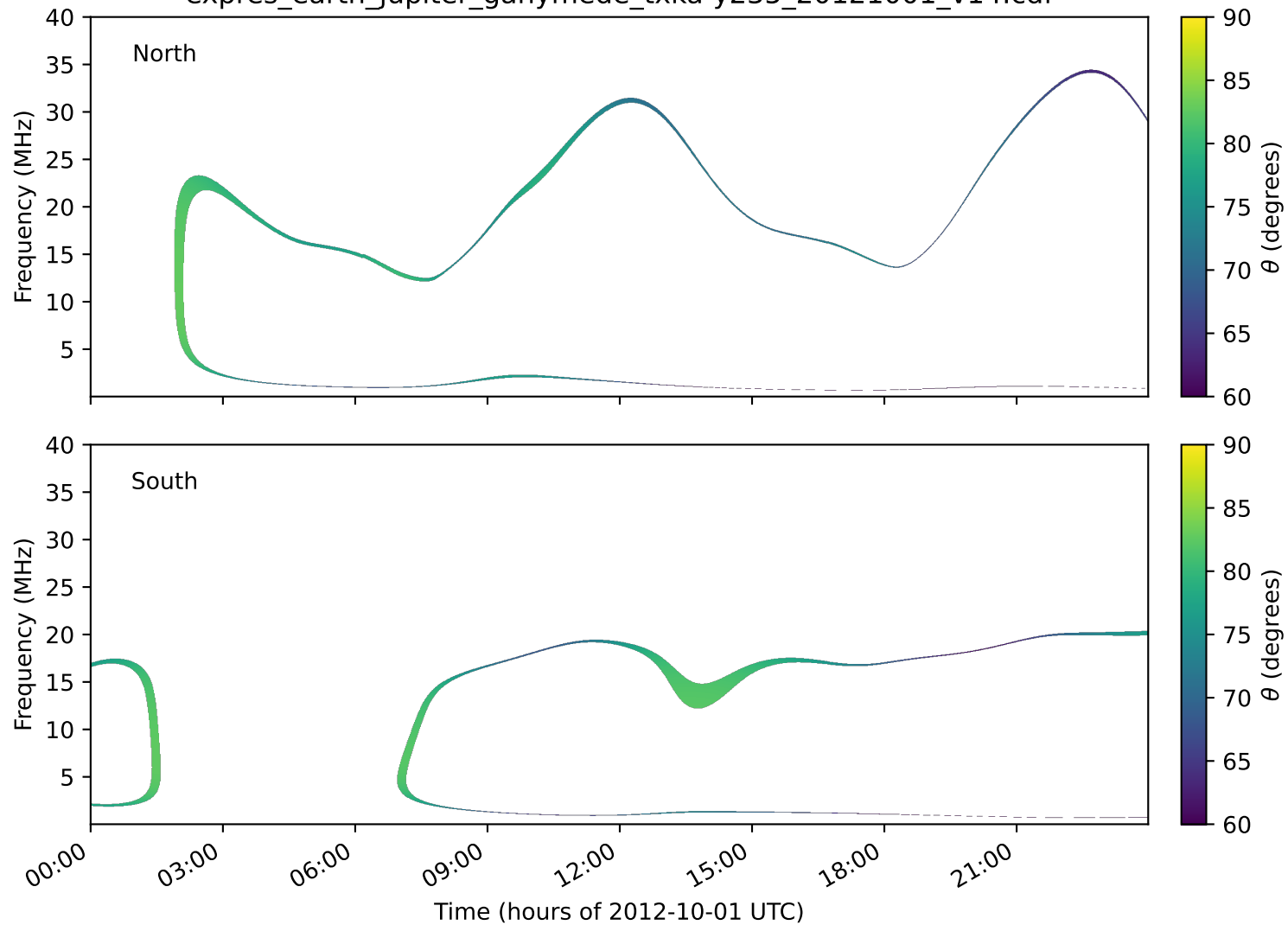
expres_earth_jupiter_ganymede_txka-y235_20121001_v14.cdf
