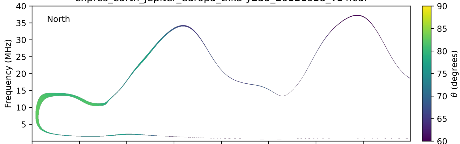
expres_earth_jupiter_europa_txka-y235_20121028_v14.cdf
