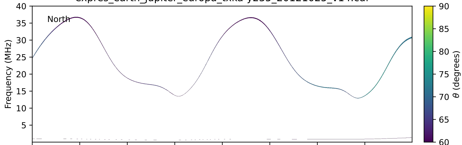
expres_earth_jupiter_europa_txka-y235_20121025_v14.cdf
