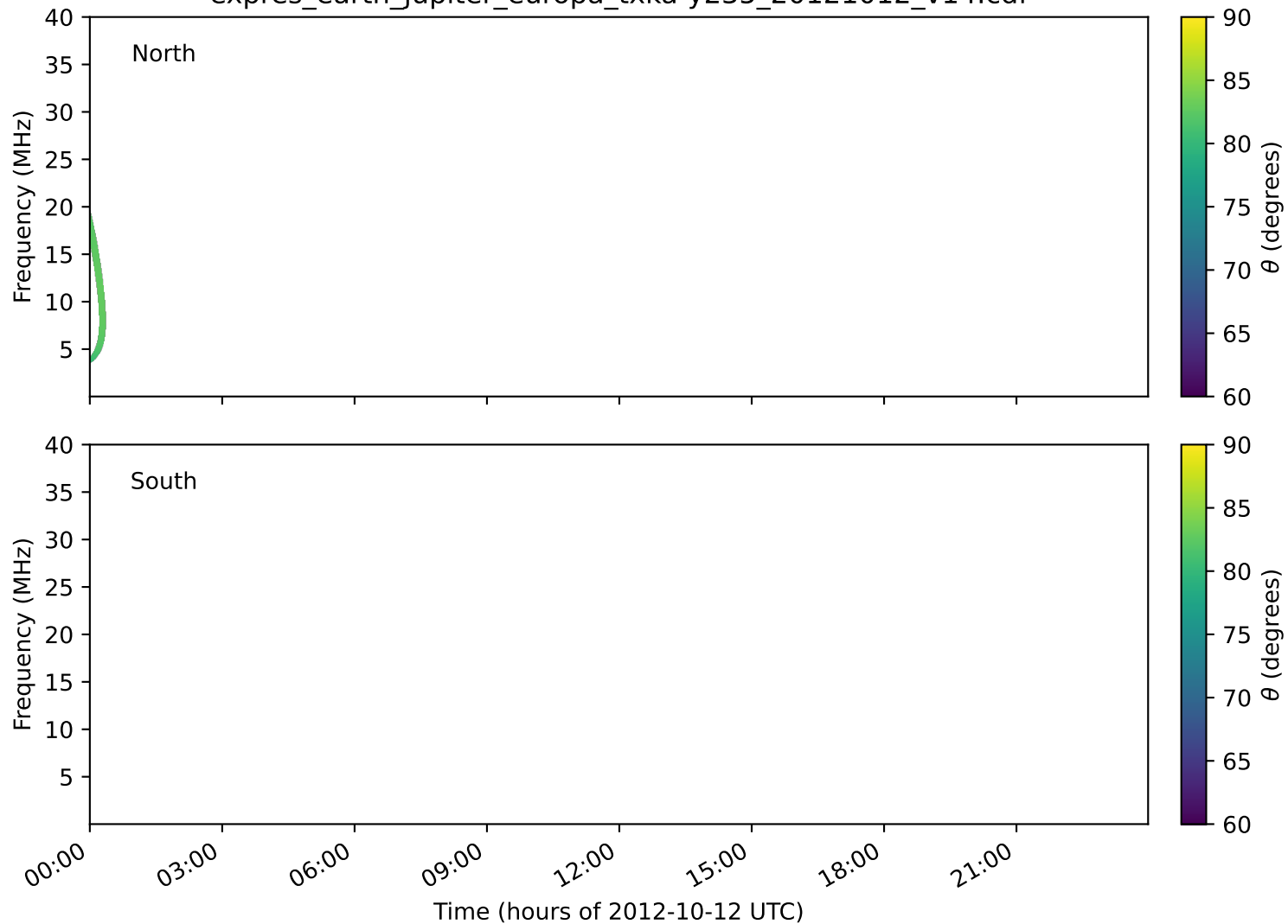
expres_earth_jupiter_europa_txka-y235_20121012_v14.cdf
