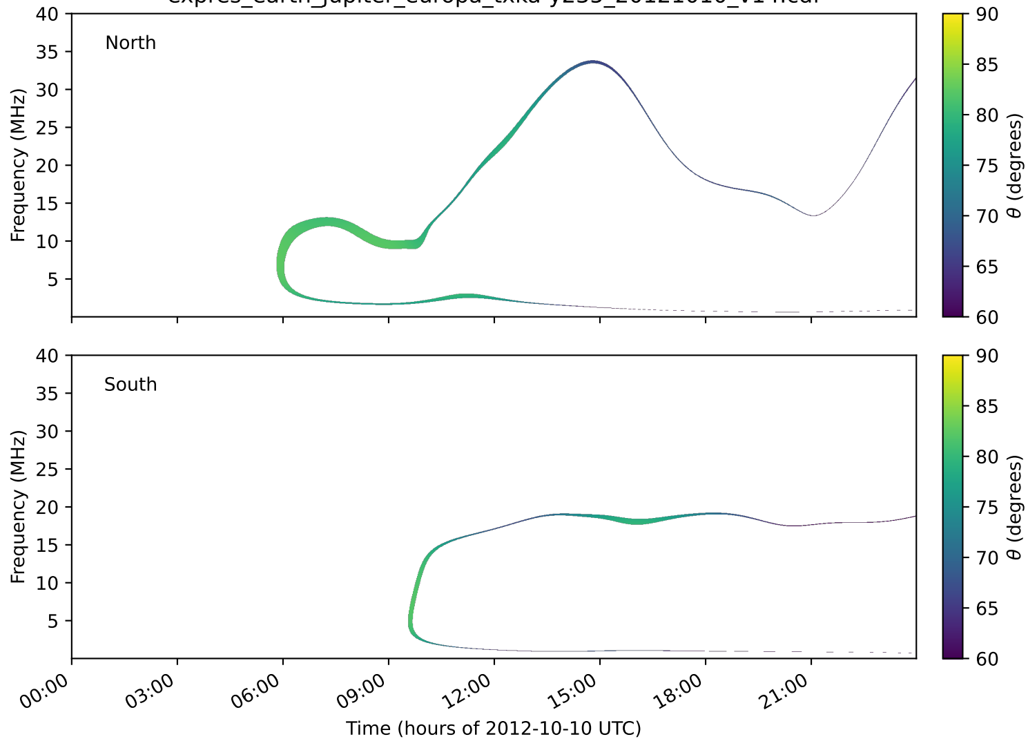
expres_earth_jupiter_europa_txka-y235_20121010_v14.cdf
