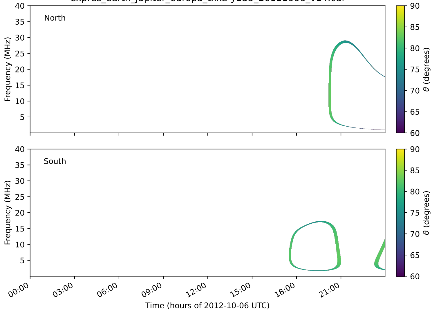
expres_earth_jupiter_europa_txka-y235_20121006_v14.cdf
