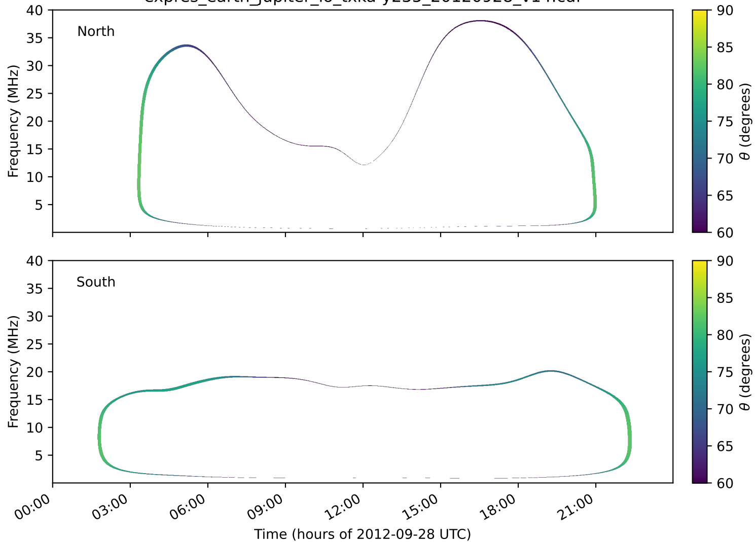
expres_earth_jupiter_io_txka-y235_20120928_v14.cdf
