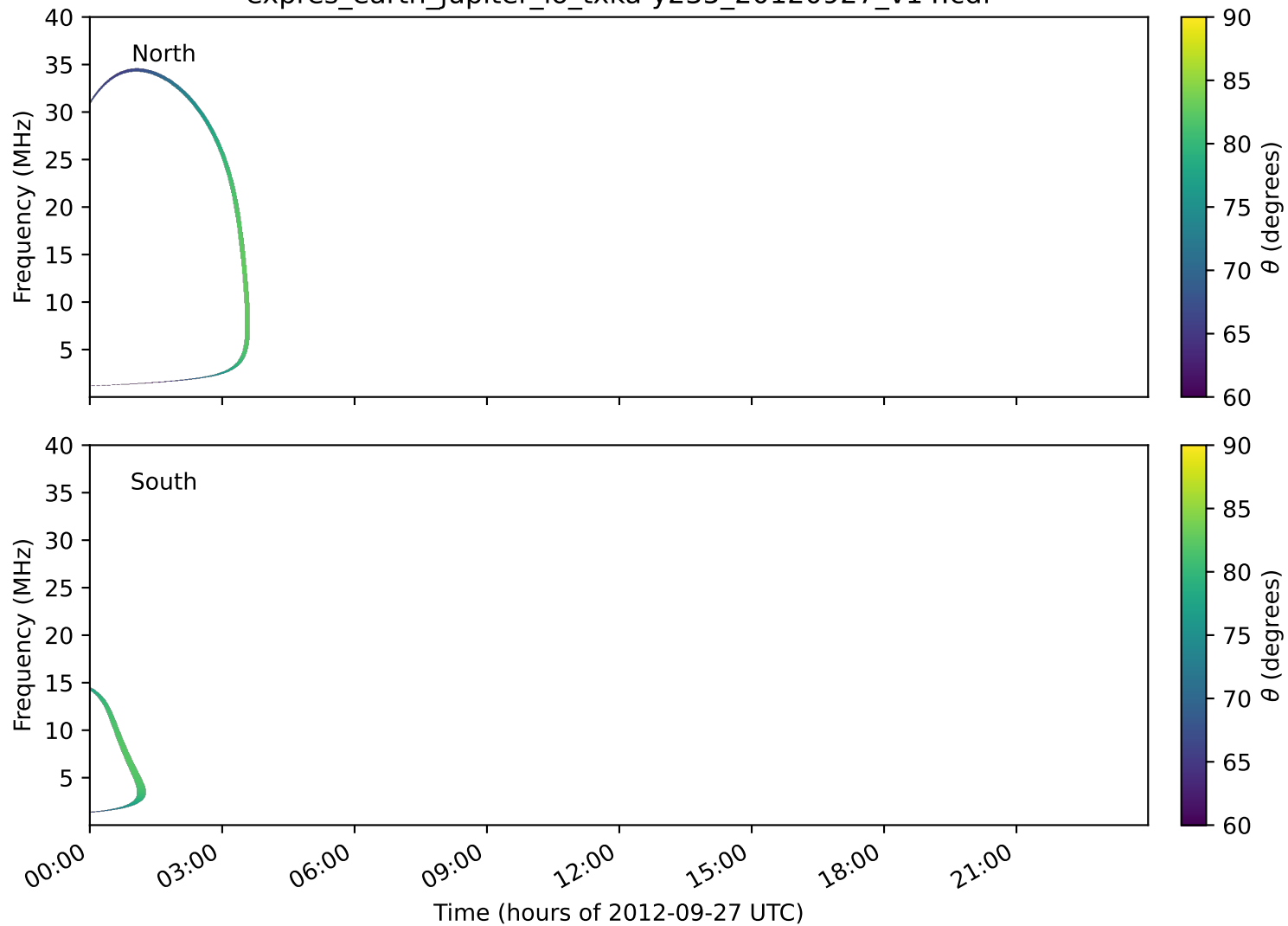
expres_earth_jupiter_io_txka-y235_20120927_v14.cdf
