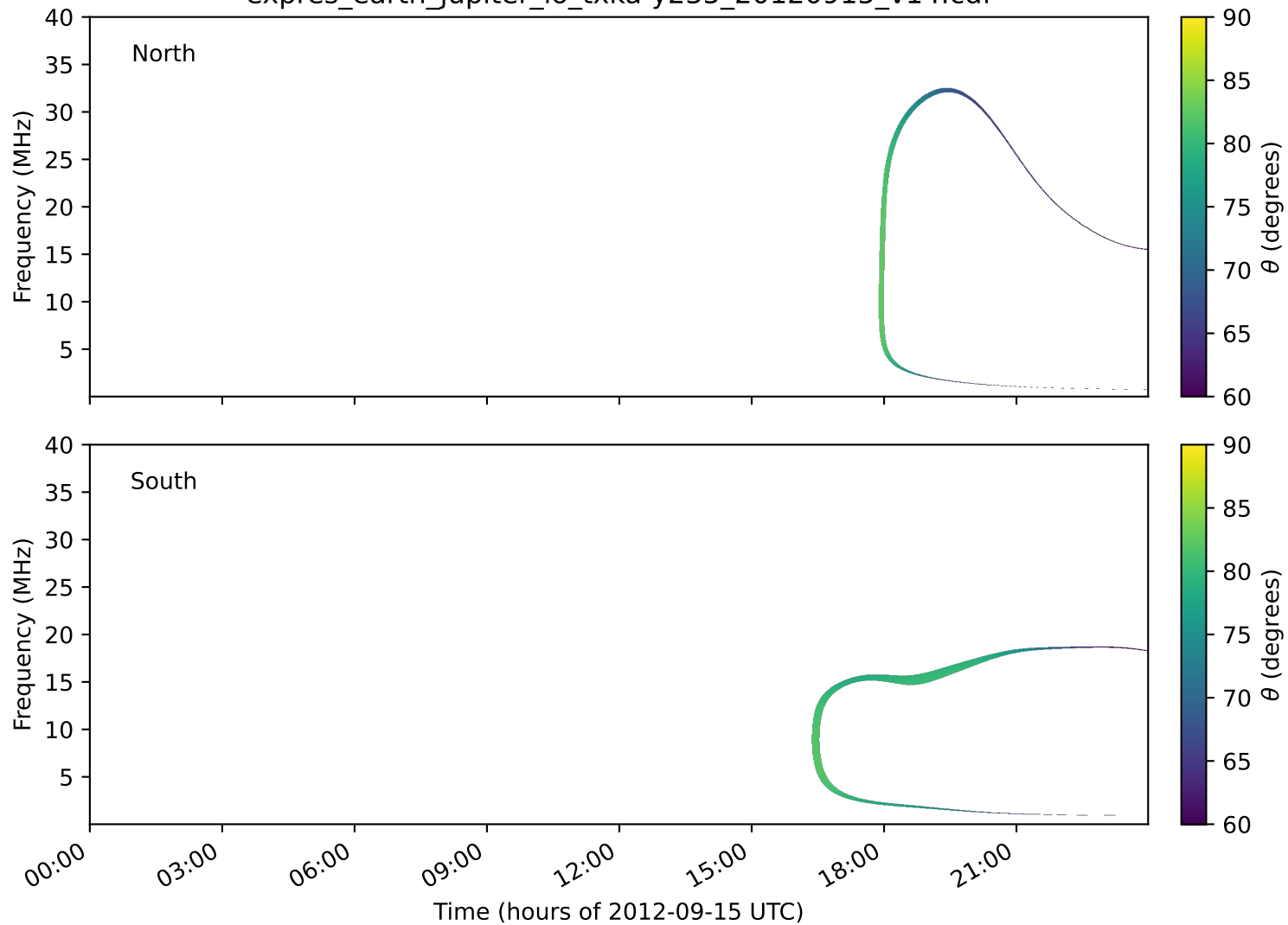
expres_earth_jupiter_io_txka-y235_20120915_v14.cdf
