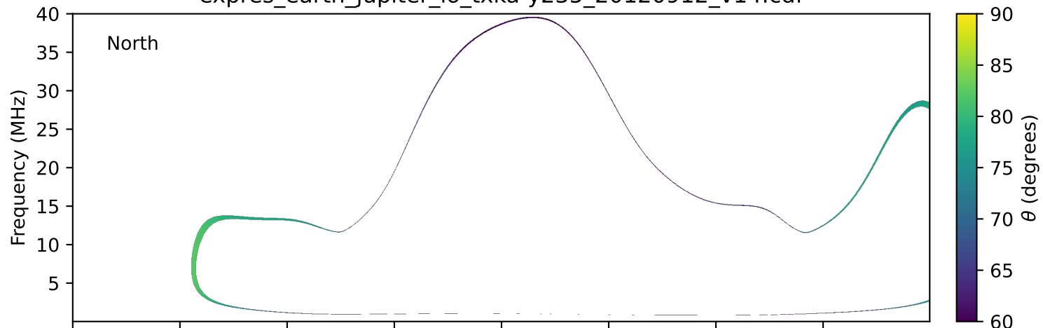
expres_earth_jupiter_io_txka-y235_20120912_v14.cdf
