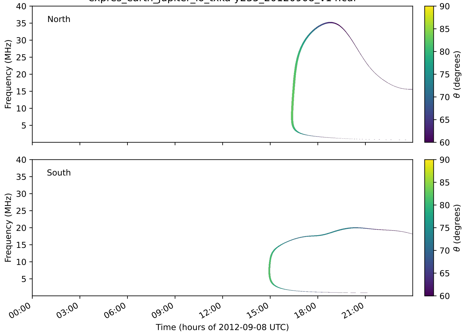
expres_earth_jupiter_io_txka-y235_20120908_v14.cdf
