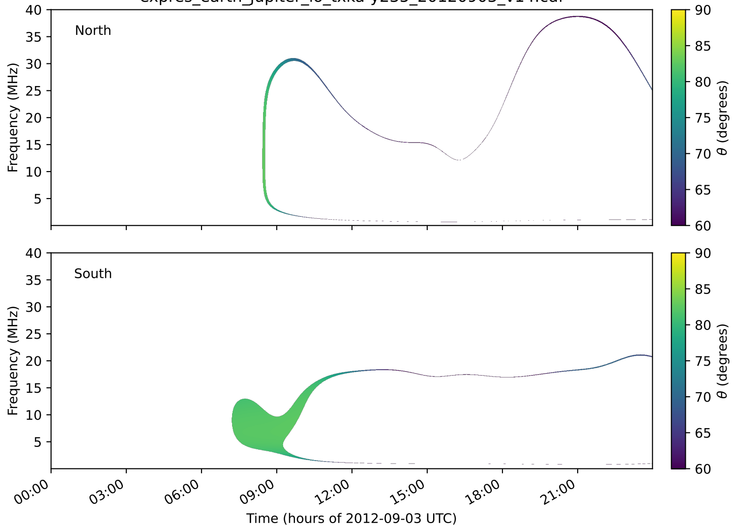
expres_earth_jupiter_io_txka-y235_20120903_v14.cdf
