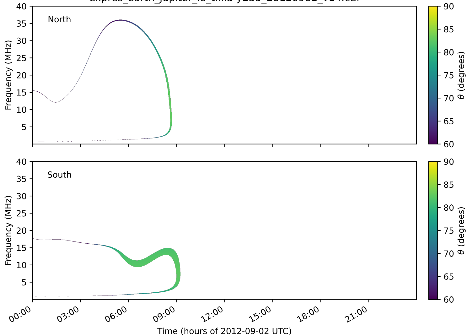
expres_earth_jupiter_io_txka-y235_20120902_v14.cdf
