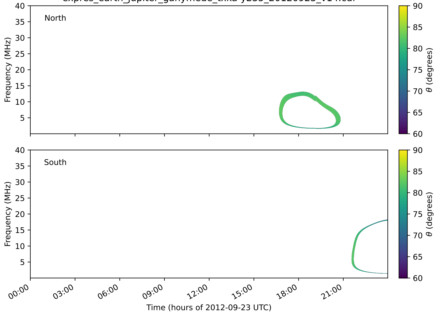
expres_earth_jupiter_ganymede_txka-y235_20120923_v14.cdf
