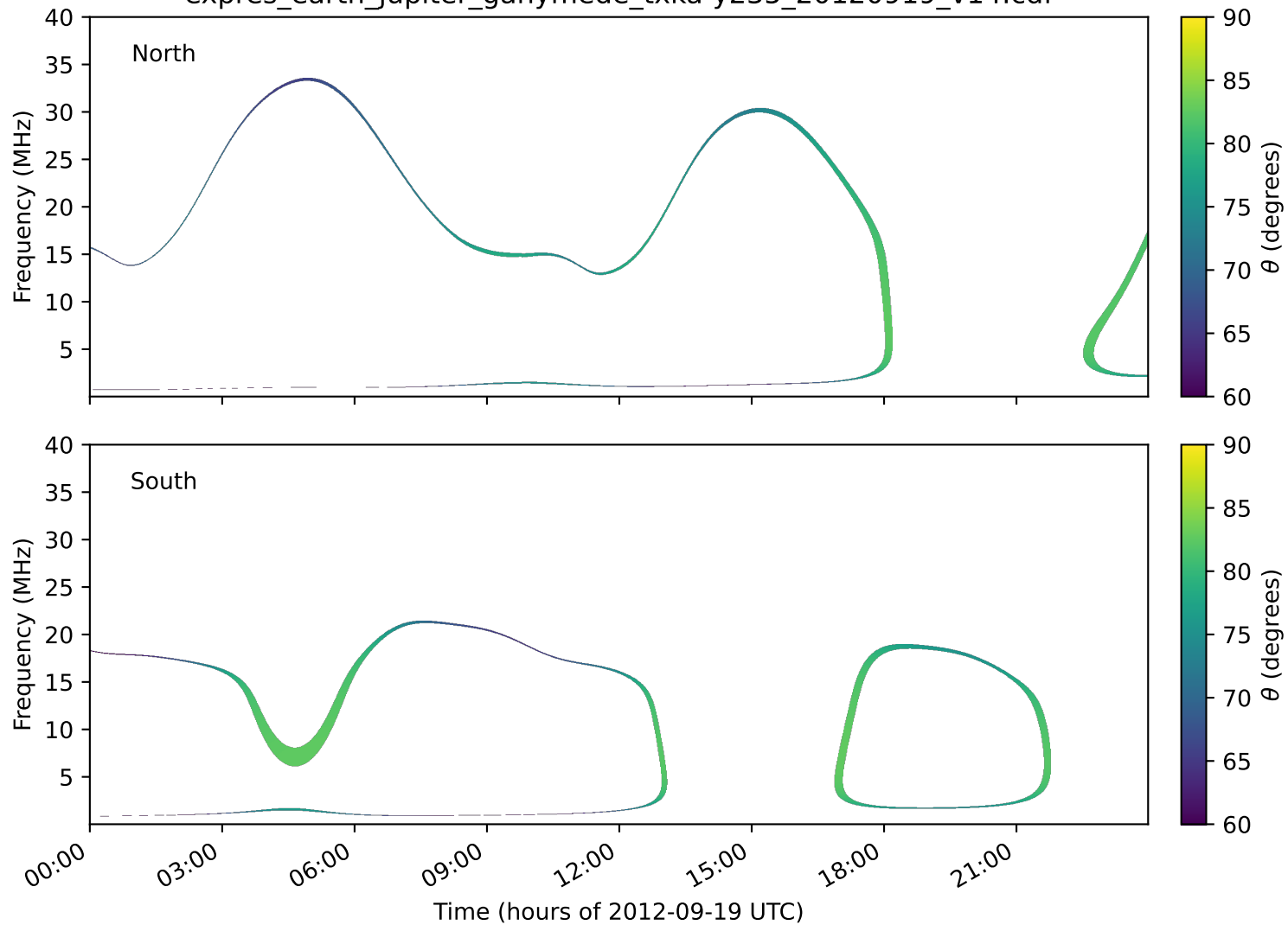
expres_earth_jupiter_ganymede_txka-y235_20120919_v14.cdf
