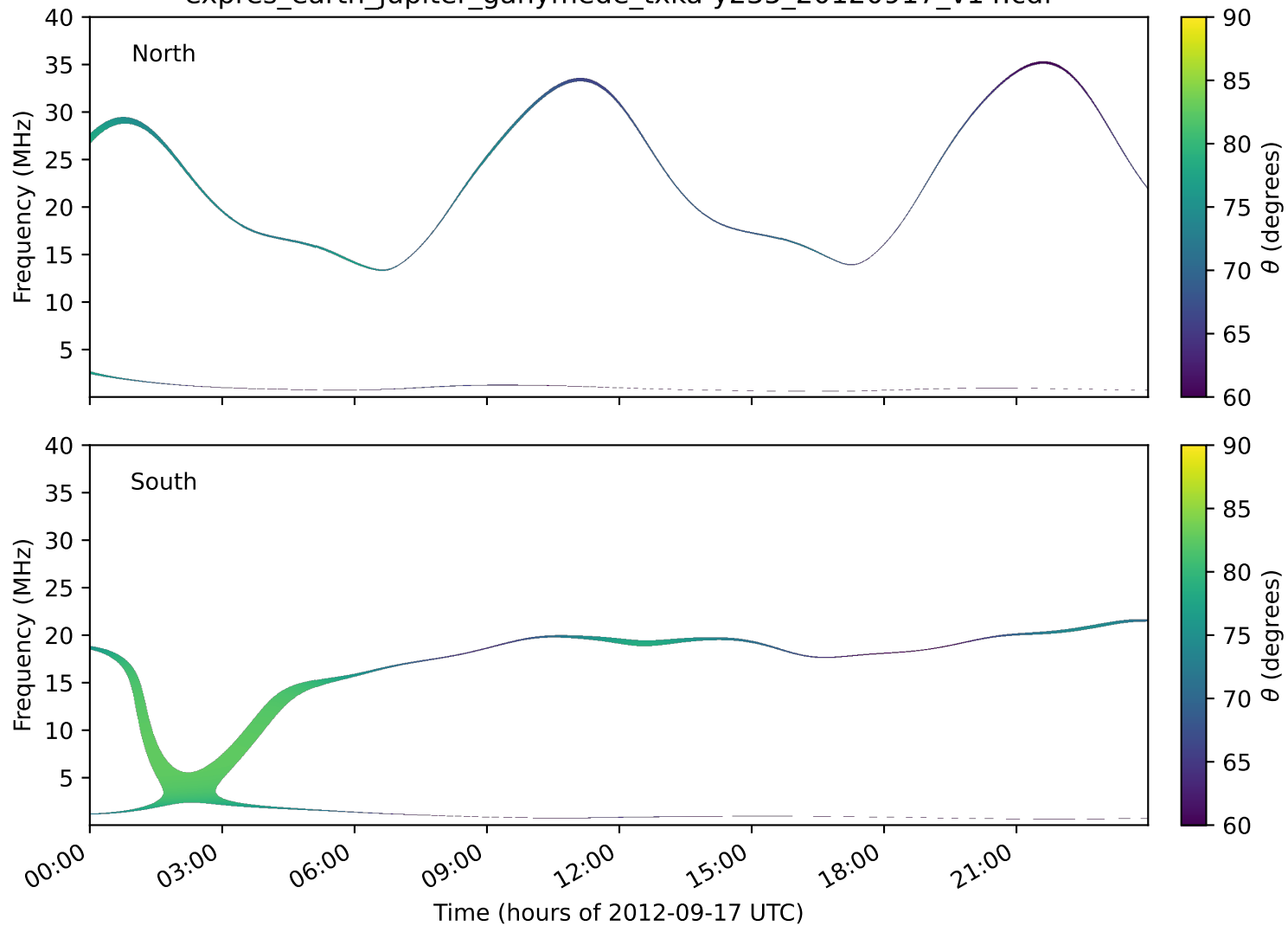
expres_earth_jupiter_ganymede_txka-y235_20120917_v14.cdf
