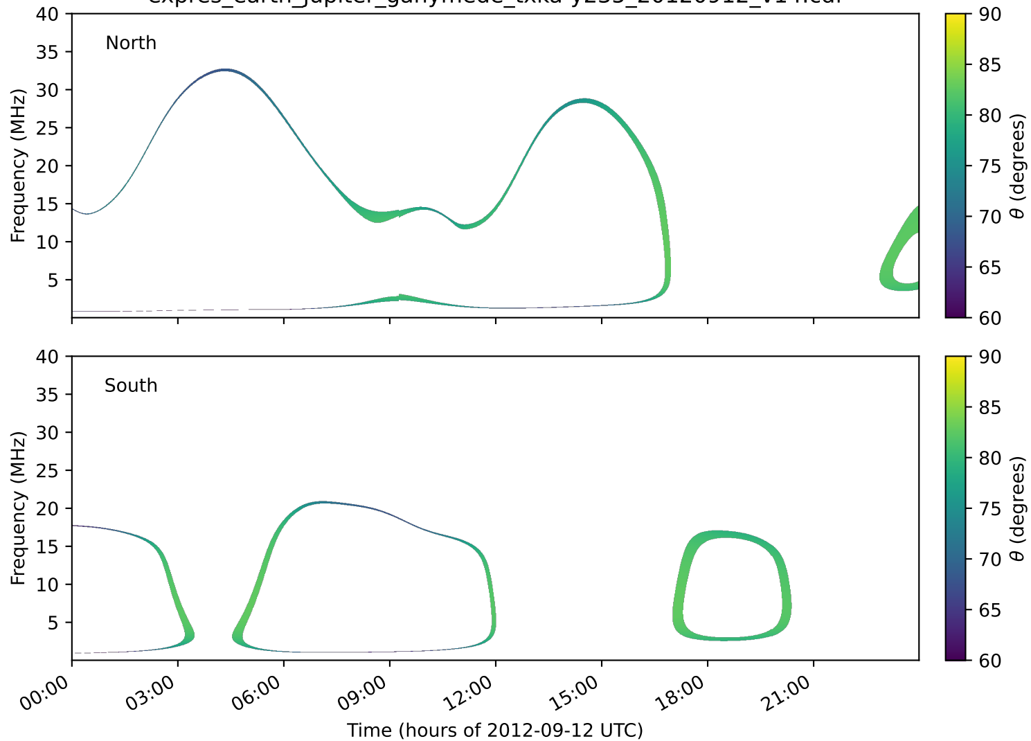
expres_earth_jupiter_ganymede_txka-y235_20120912_v14.cdf
