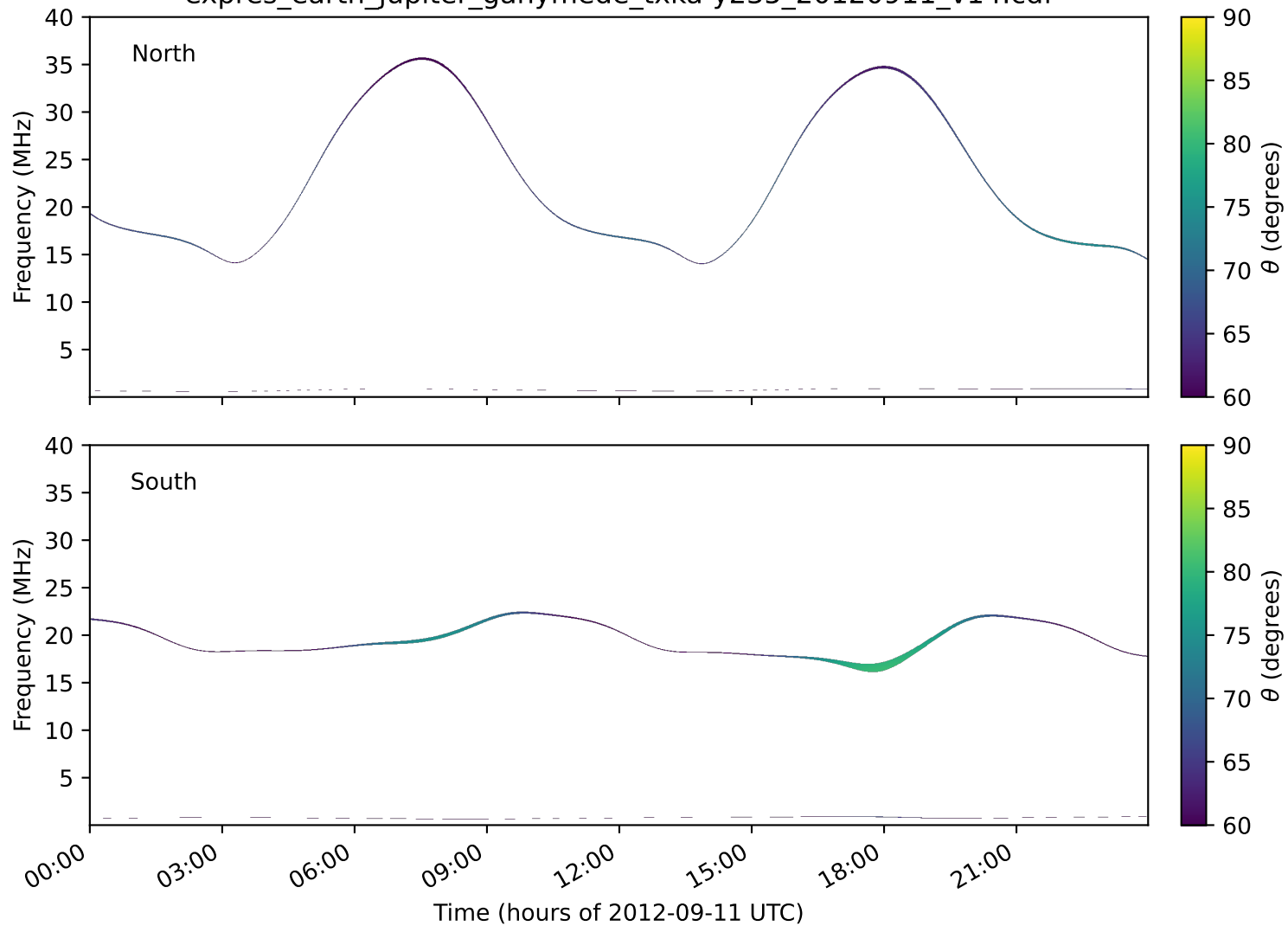
expres_earth_jupiter_ganymede_txka-y235_20120911_v14.cdf
