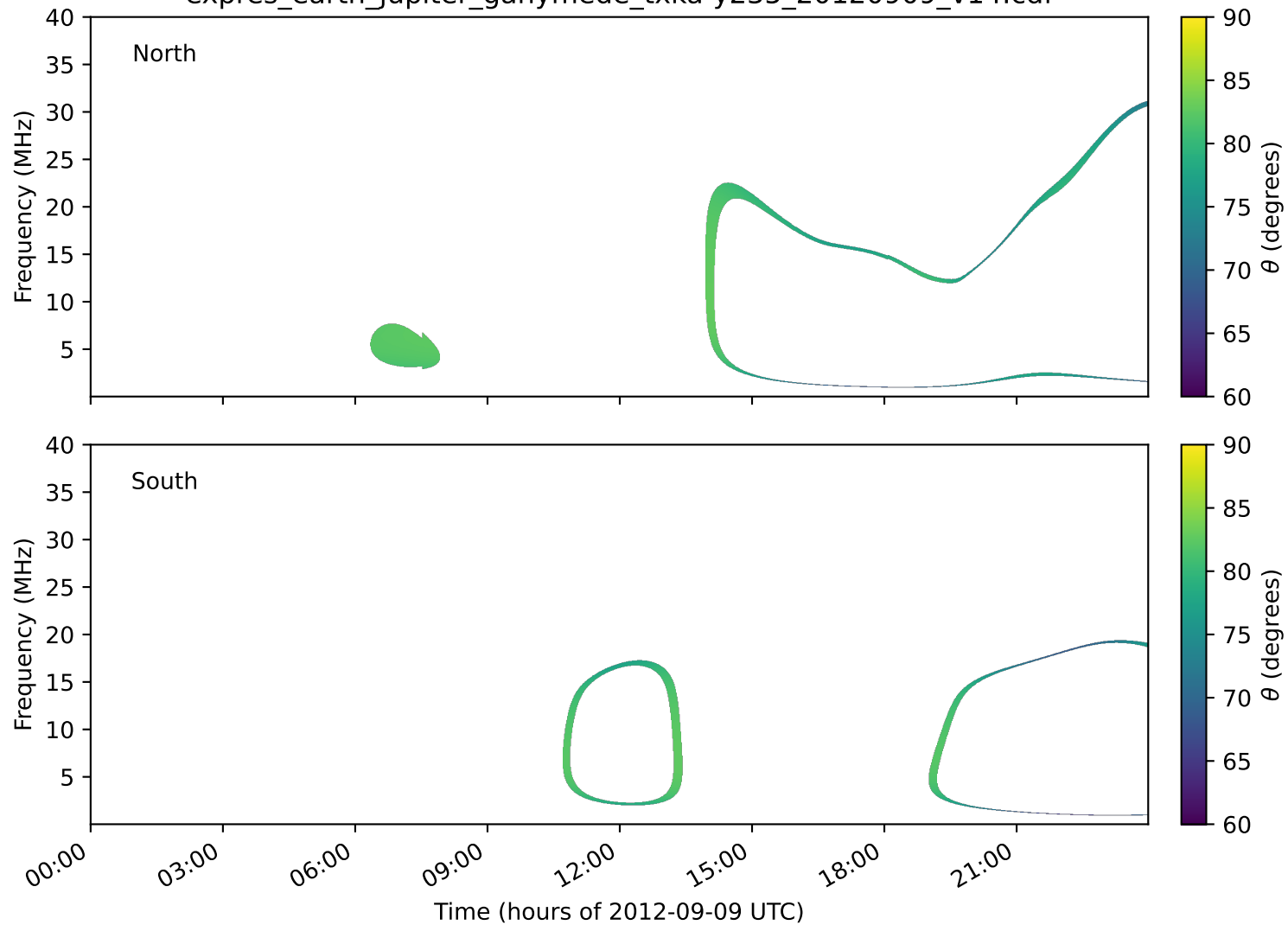
expres_earth_jupiter_ganymede_txka-y235_20120909_v14.cdf
