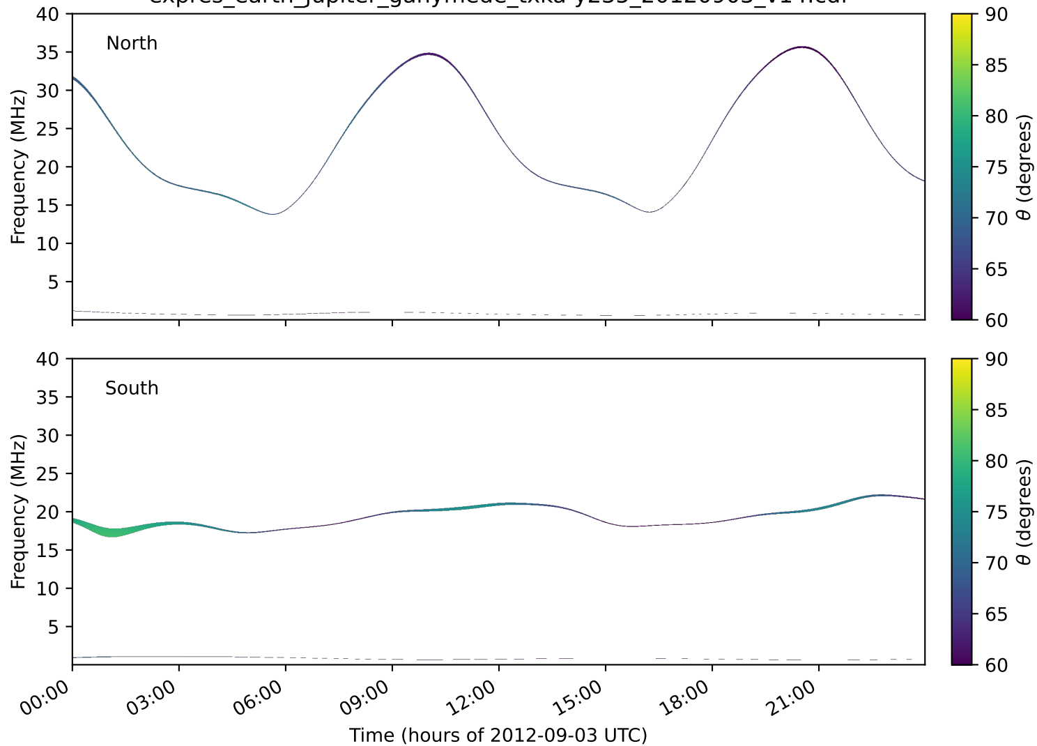
expres_earth_jupiter_ganymede_txka-y235_20120903_v14.cdf
