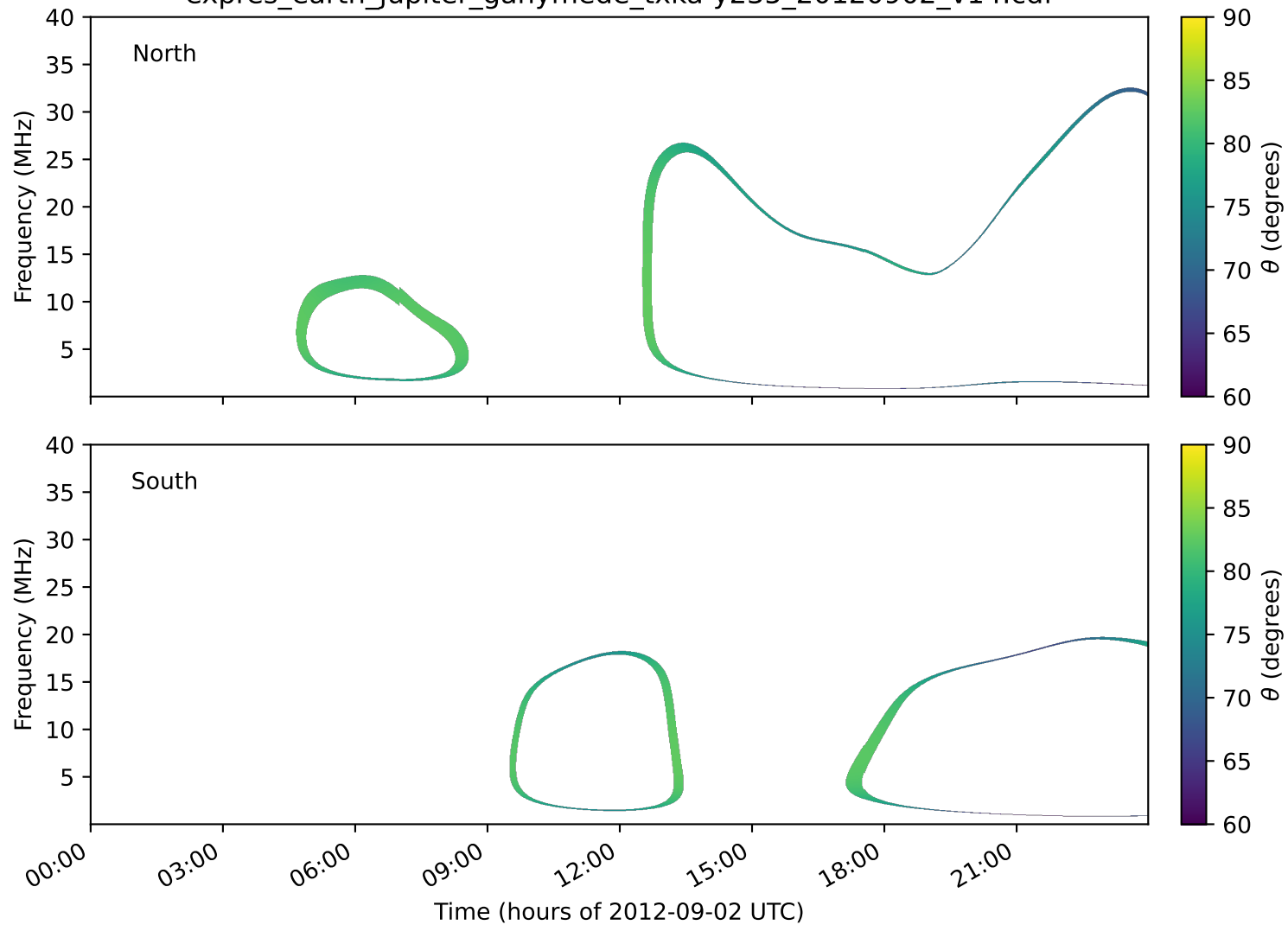
expres_earth_jupiter_ganymede_txka-y235_20120902_v14.cdf
