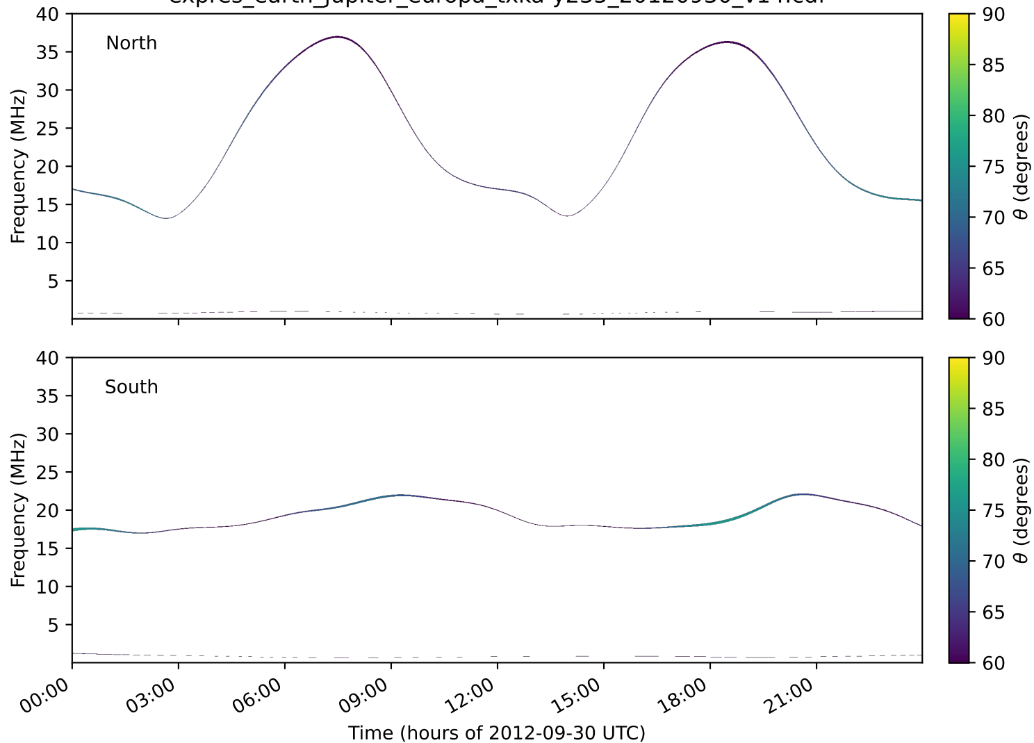
expres_earth_jupiter_europa_txka-y235_20120930_v14.cdf
