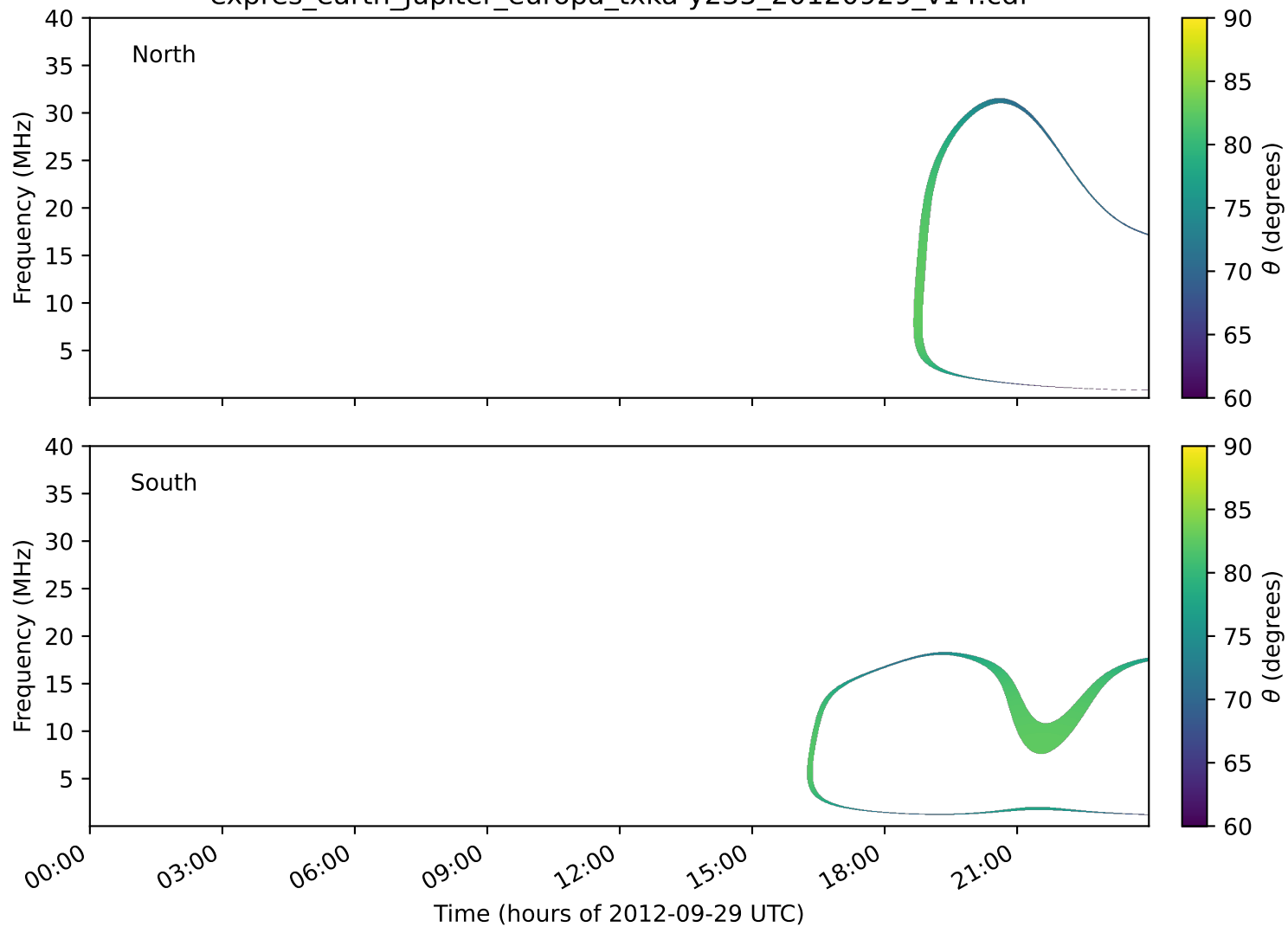
expres_earth_jupiter_europa_txka-y235_20120929_v14.cdf
