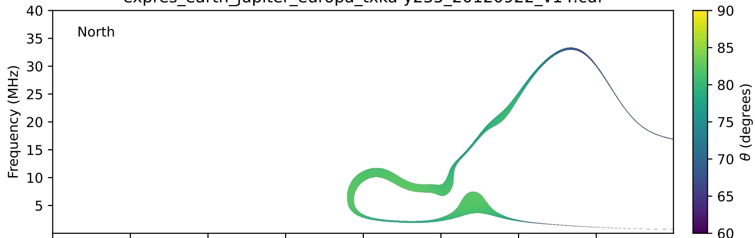
expres_earth_jupiter_europa_txka-y235_20120922_v14.cdf
