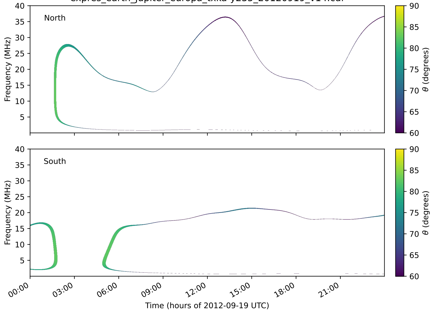
expres_earth_jupiter_europa_txka-y235_20120919_v14.cdf
