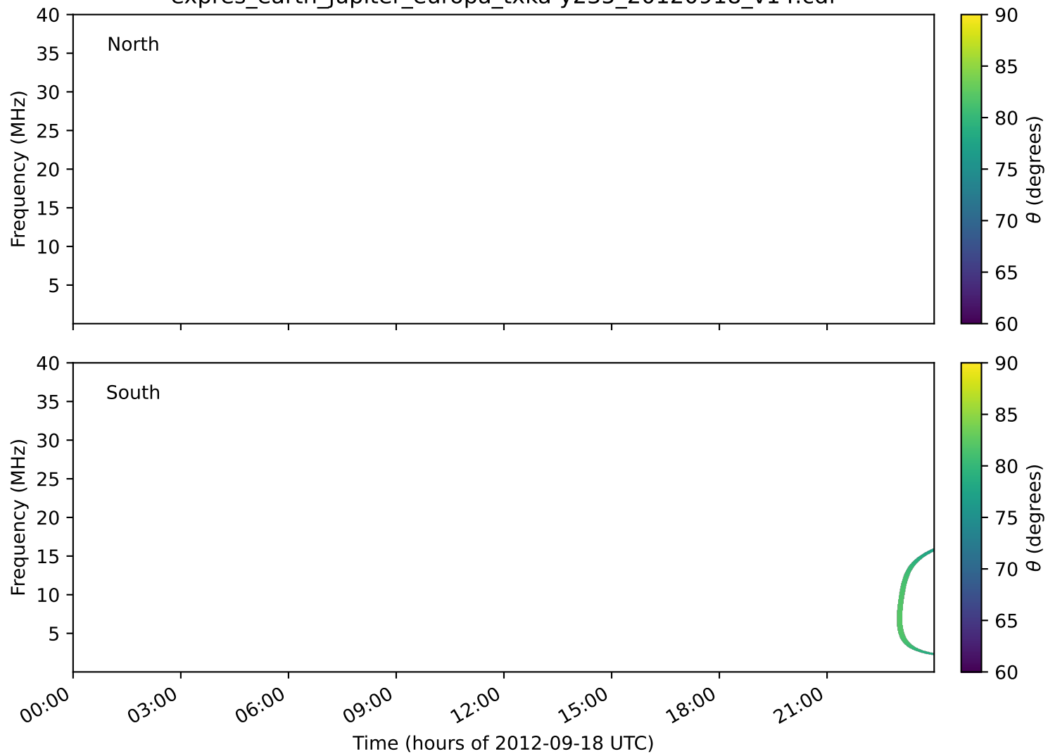
expres_earth_jupiter_europa_txka-y235_20120918_v14.cdf
