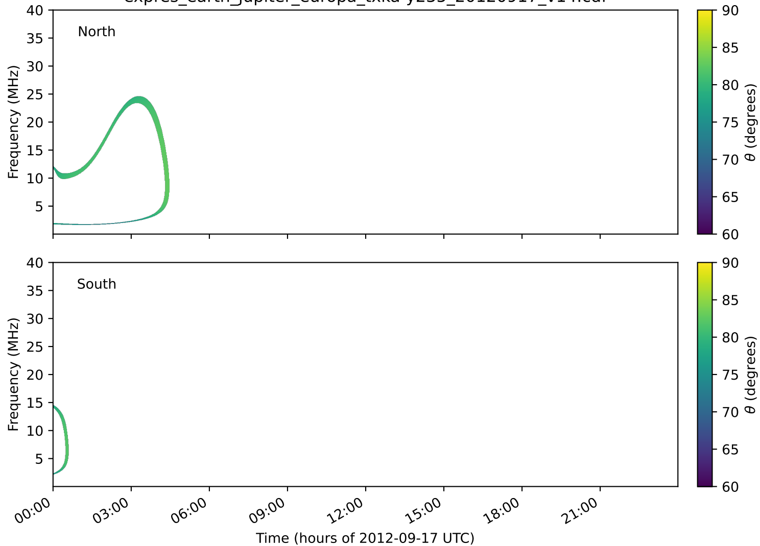
expres_earth_jupiter_europa_txka-y235_20120917_v14.cdf
