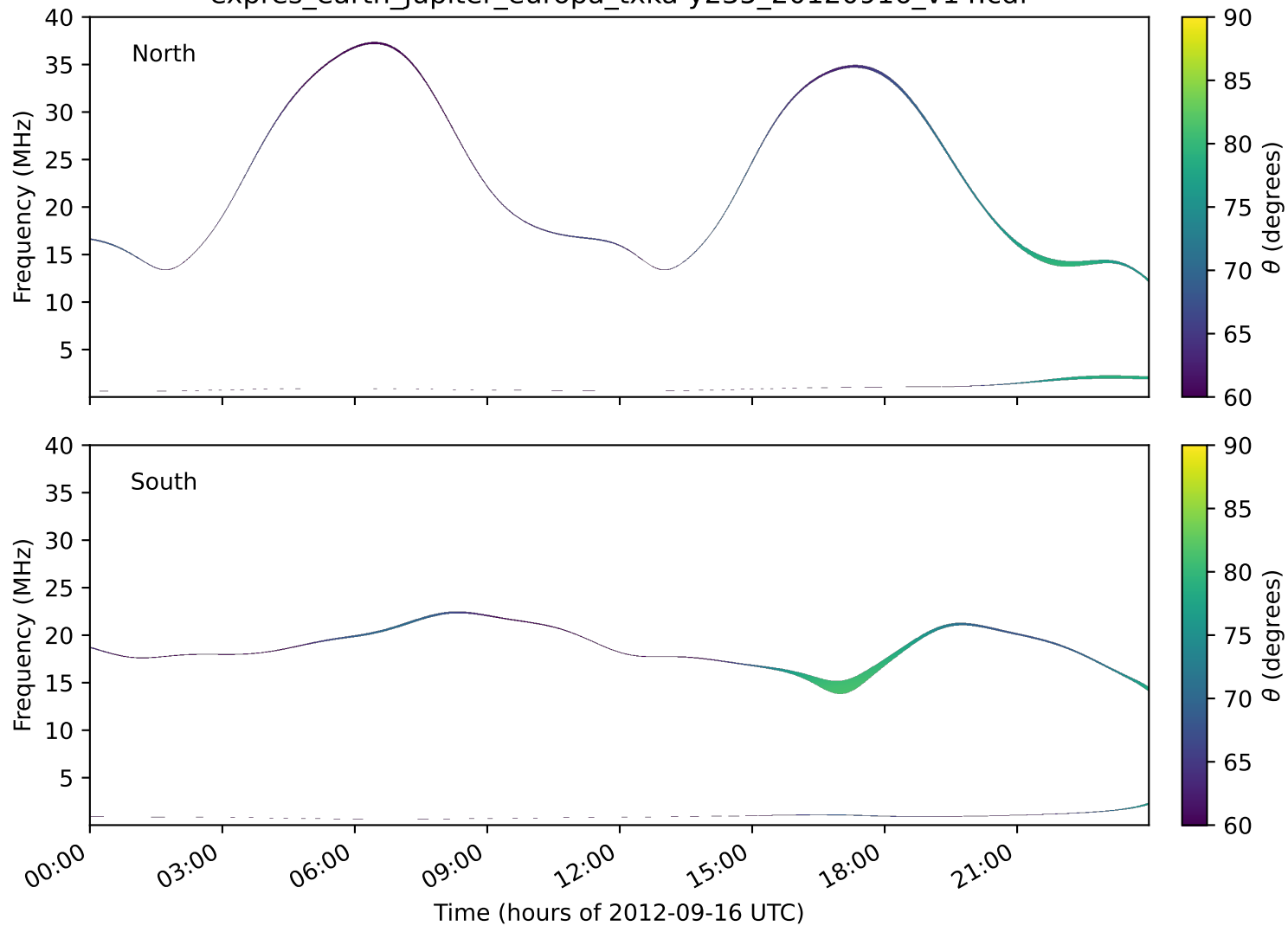
expres_earth_jupiter_europa_txka-y235_20120916_v14.cdf
