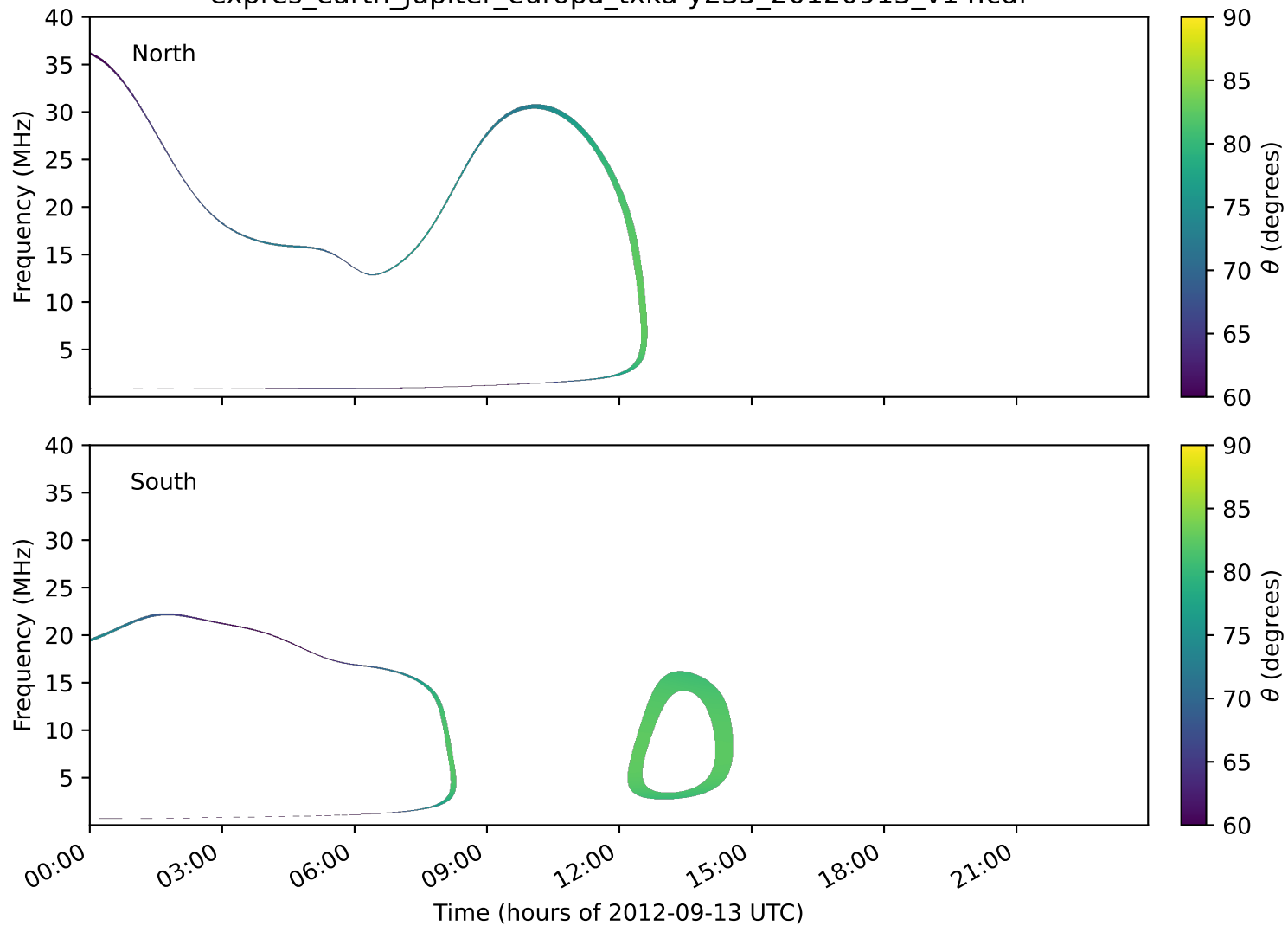
expres_earth_jupiter_europa_txka-y235_20120913_v14.cdf
