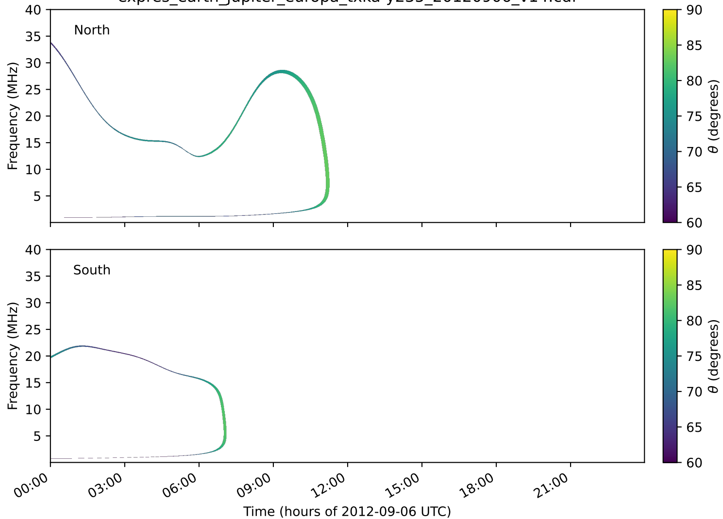
expres_earth_jupiter_europa_txka-y235_20120906_v14.cdf
