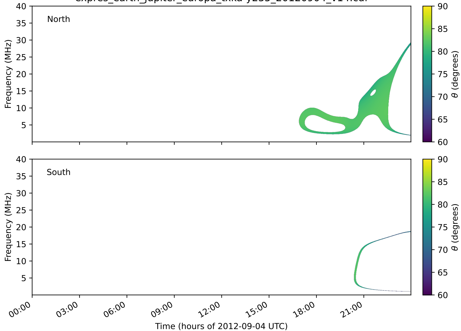
expres_earth_jupiter_europa_txka-y235_20120904_v14.cdf
