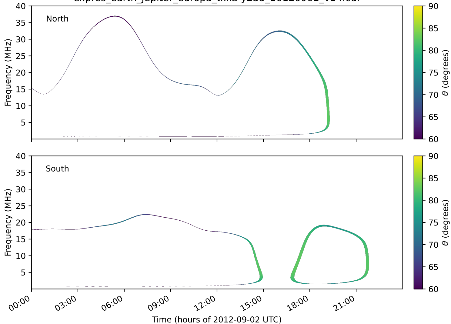
expres_earth_jupiter_europa_txka-y235_20120902_v14.cdf
