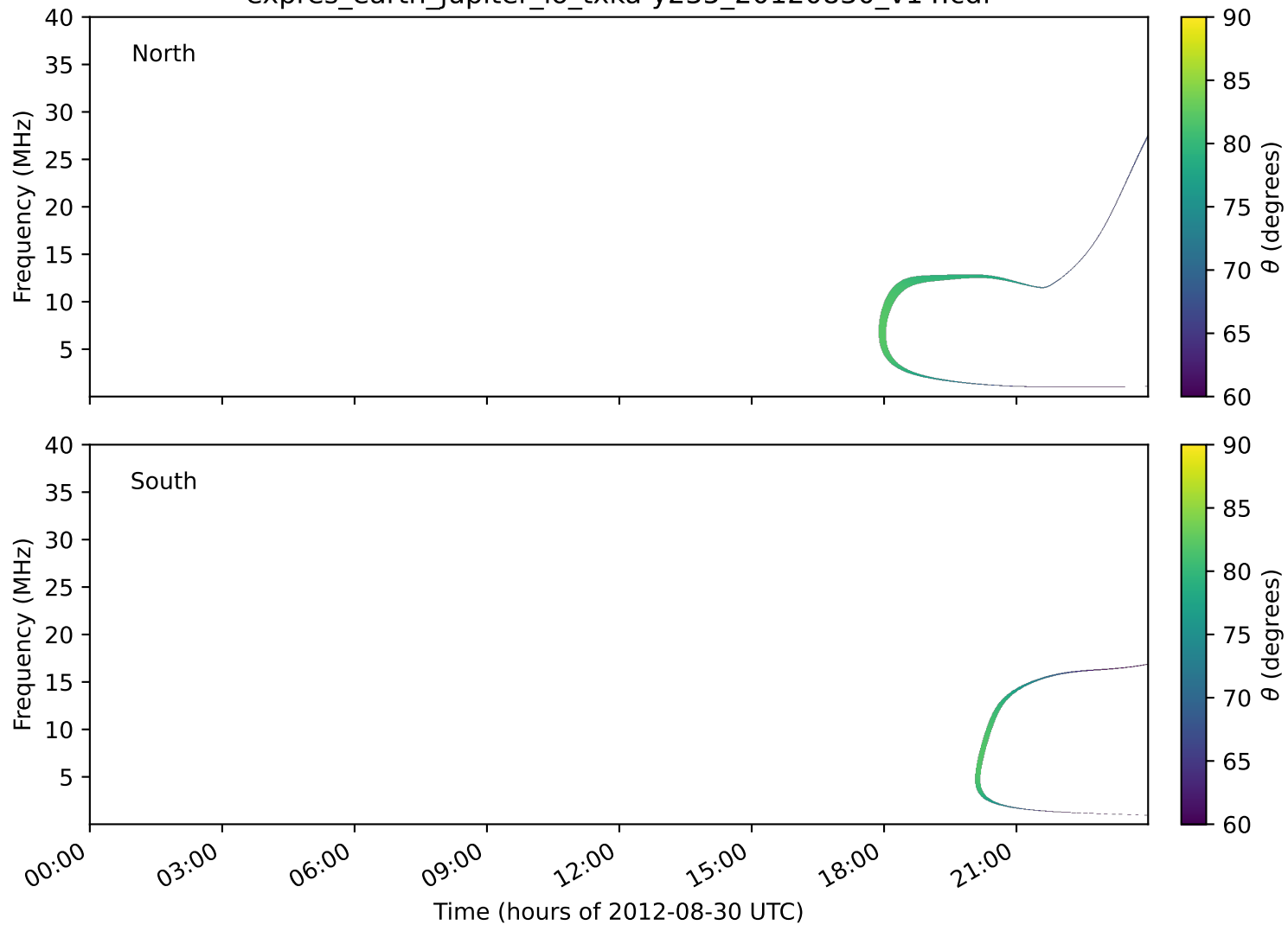
expres_earth_jupiter_io_txka-y235_20120830_v14.cdf
