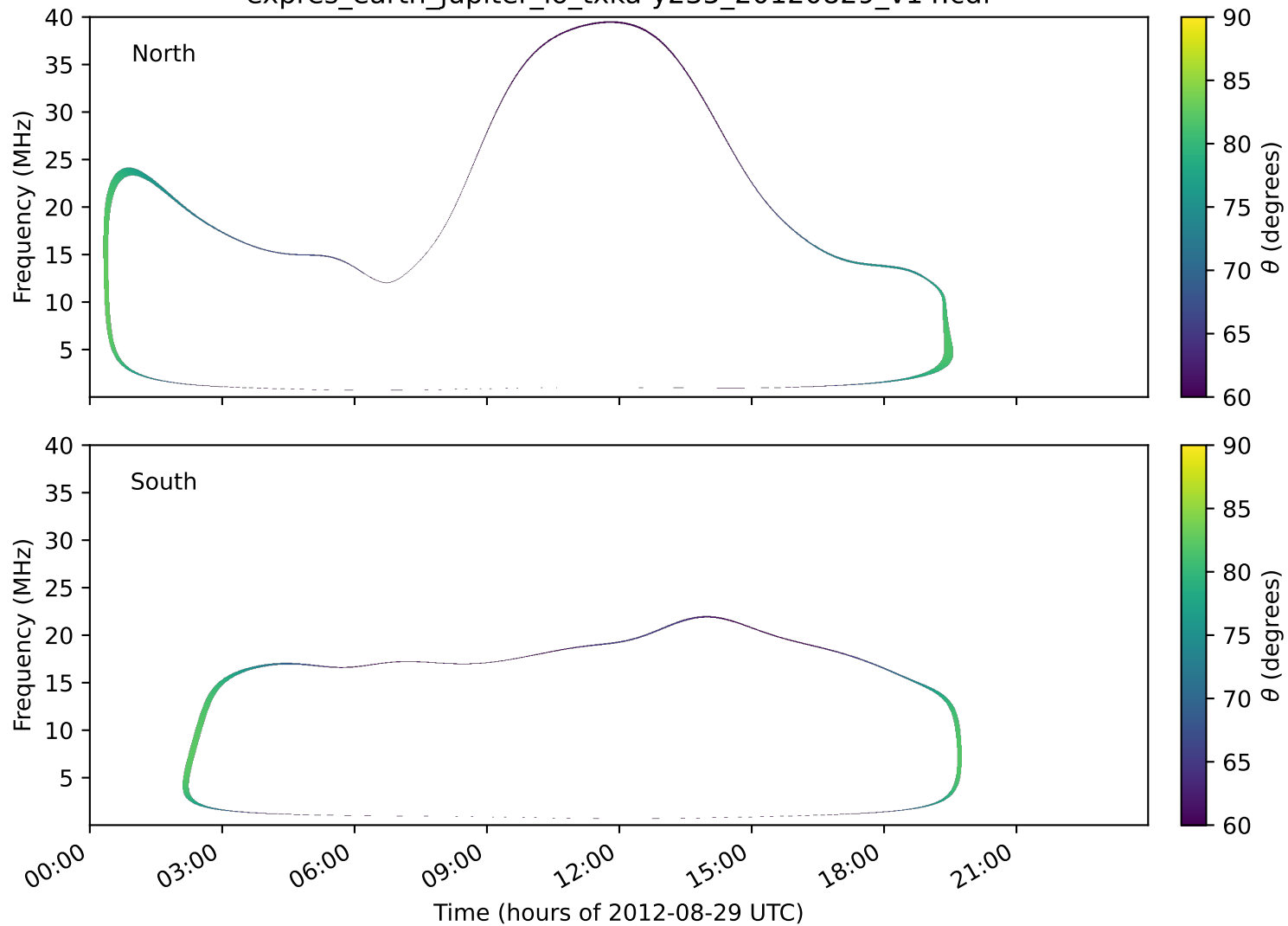
expres_earth_jupiter_io_txka-y235_20120829_v14.cdf
