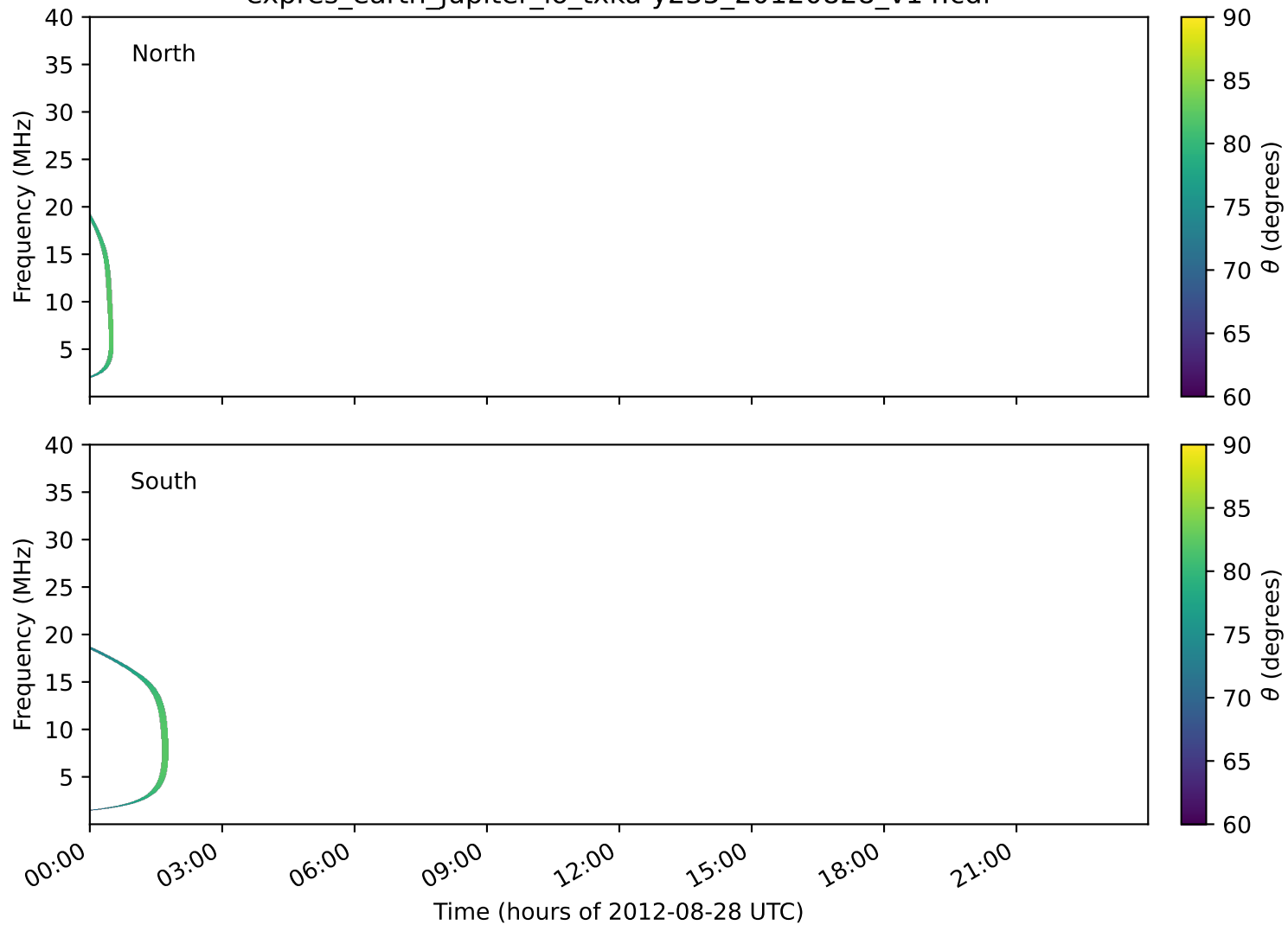
expres_earth_jupiter_io_txka-y235_20120828_v14.cdf
