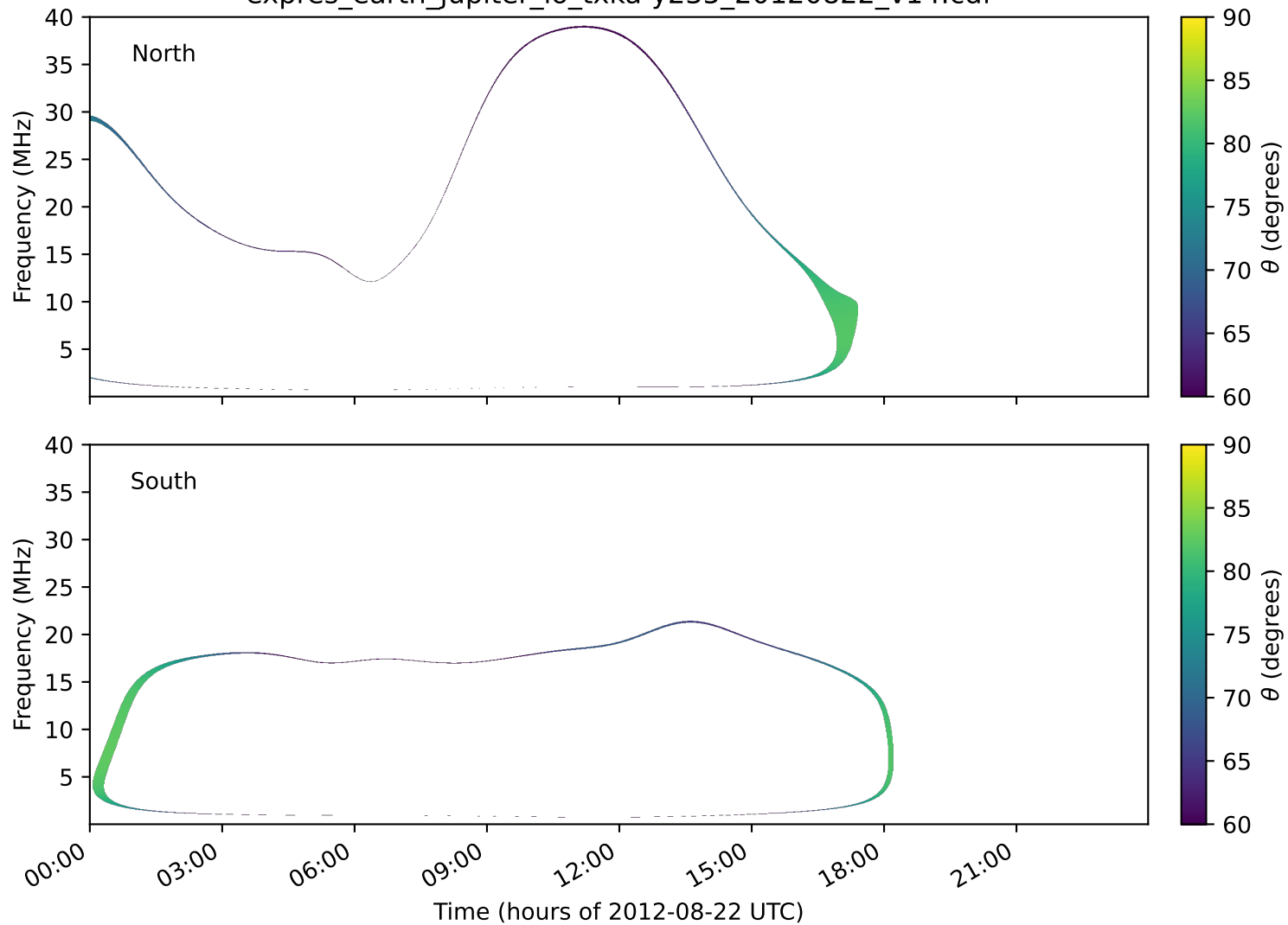
expres_earth_jupiter_io_txka-y235_20120822_v14.cdf
