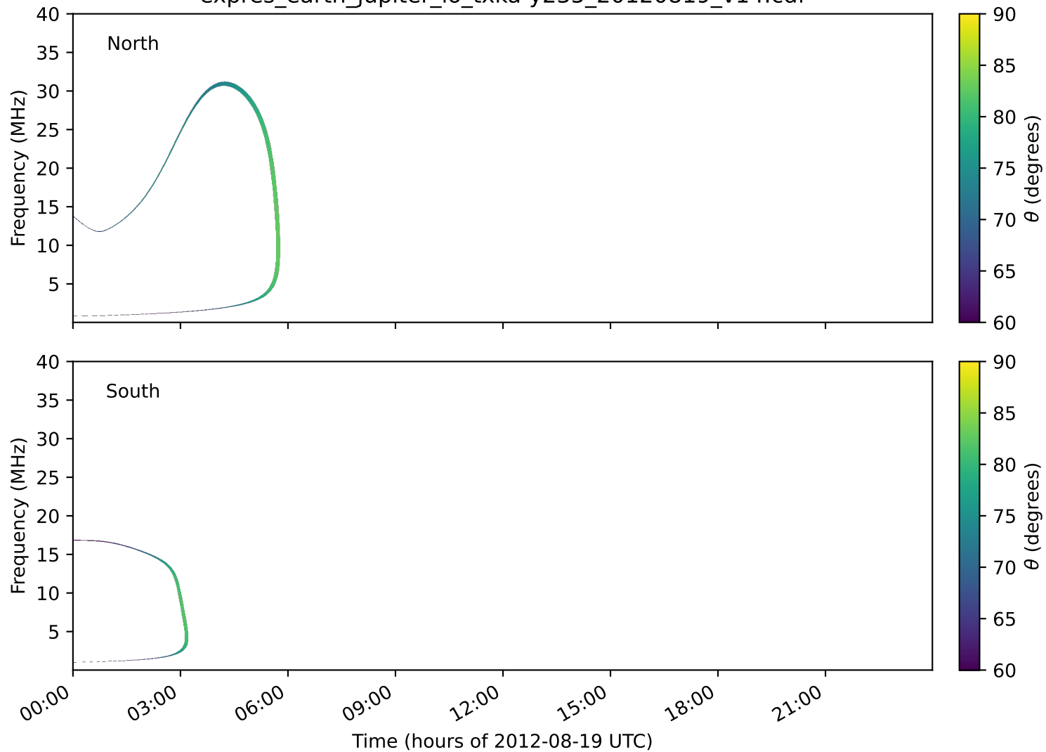
expres_earth_jupiter_io_txka-y235_20120819_v14.cdf
