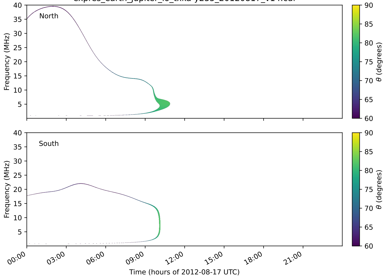
expres_earth_jupiter_io_txka-y235_20120817_v14.cdf
